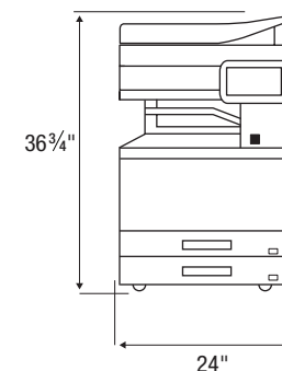
Main Unit + MX-TU16 + MX-DE29N (1 additional drawer – for wheelchair access) 1,200-sheet maximum
